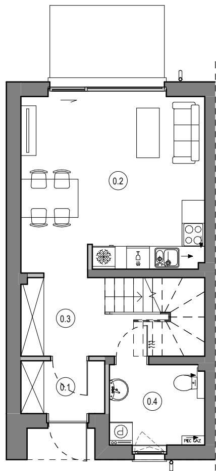
PARTER
